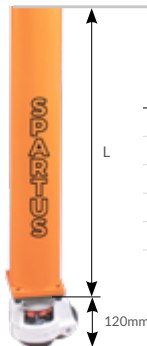
LEG WITH WHEEL
